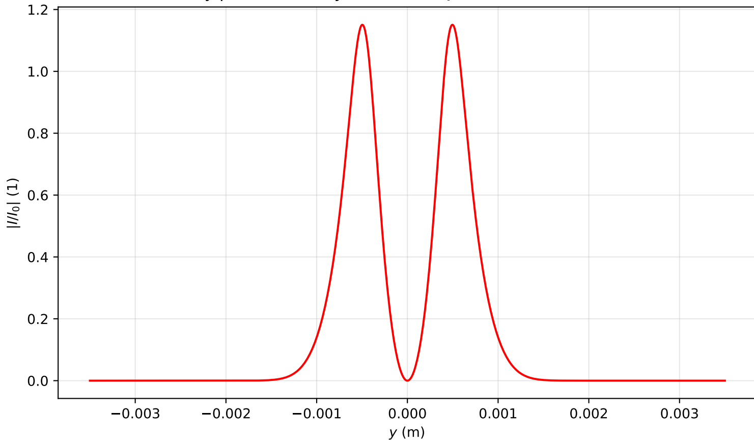
Intensity profile I(x=0, y, z=0.239)/I_0 , \text{Pin}=8.0\text{Pcr} , artificial time
